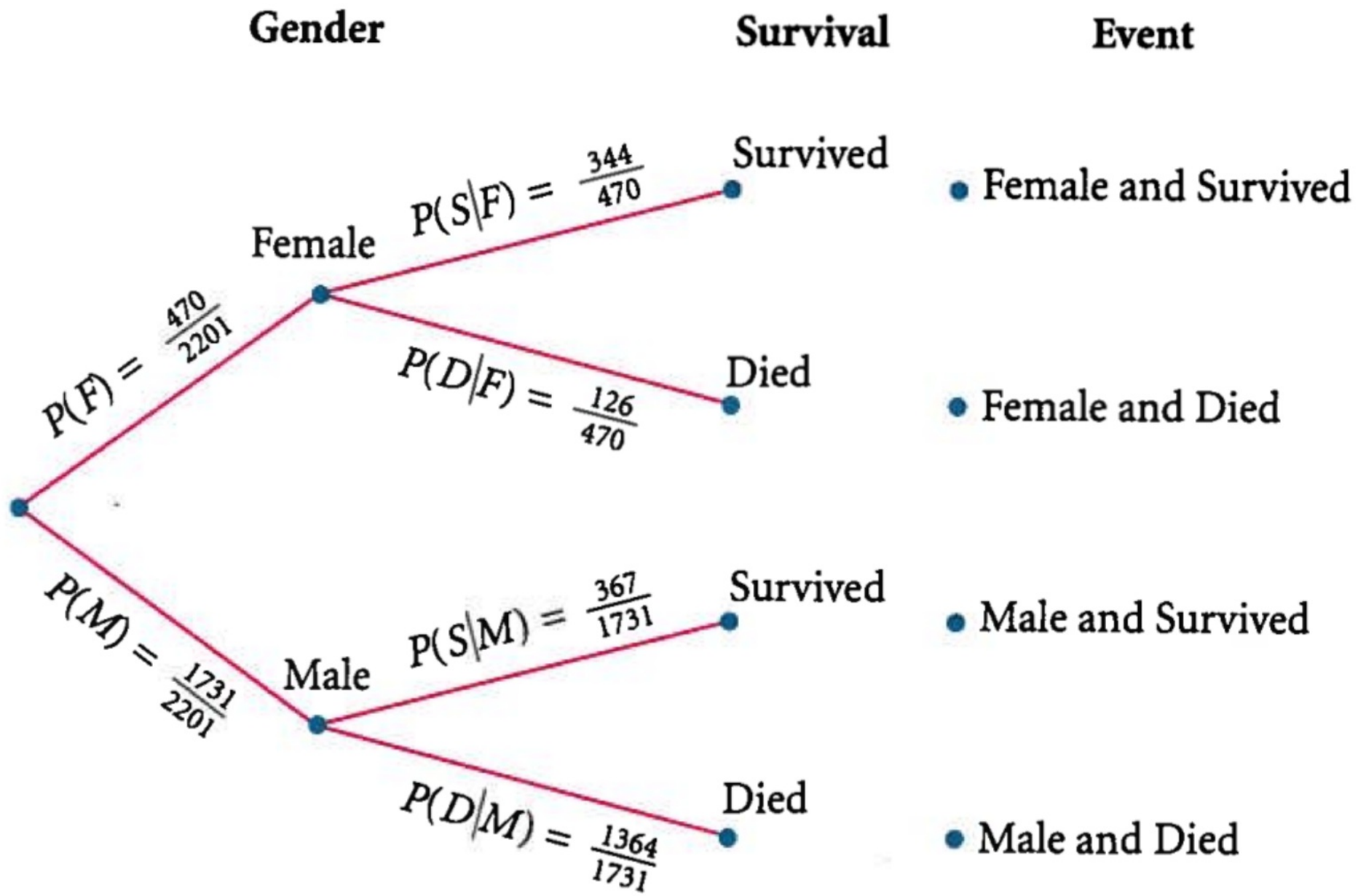
Display 5.40 Tree diagram for the Titanic data.
